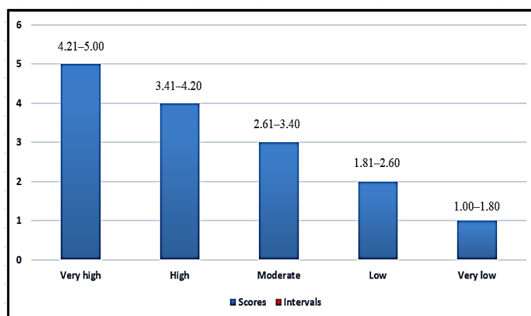
Figure 2: A Scale and Score Interval is Used to Evaluate Scale Data.
