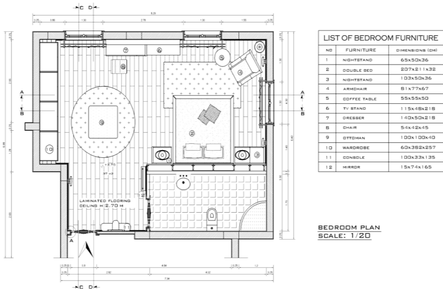
Figure 2. The task of the bedroom plan drawing sheet that was given to the students
